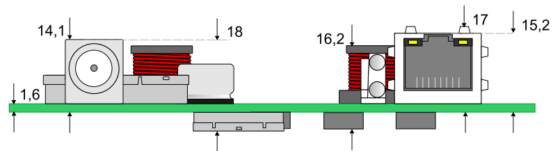
Dimensions Components sideview PCB front
