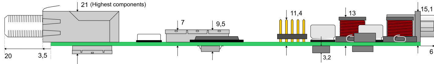
Dimensions Components sideview PCB longest side
